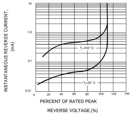
FIG.4-TYPICAL REVERSE CHARACTERISTICS
